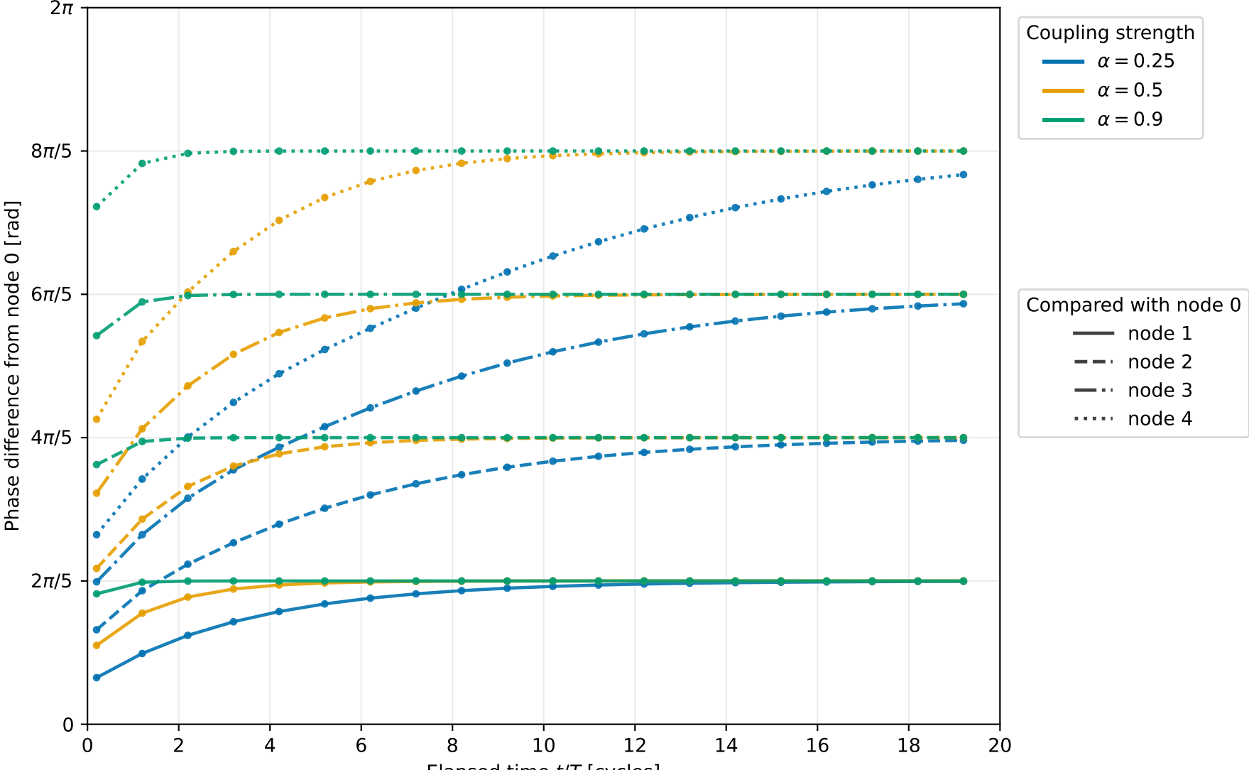
PCO-D phase difference ( N = 5, r = 1/5 )
