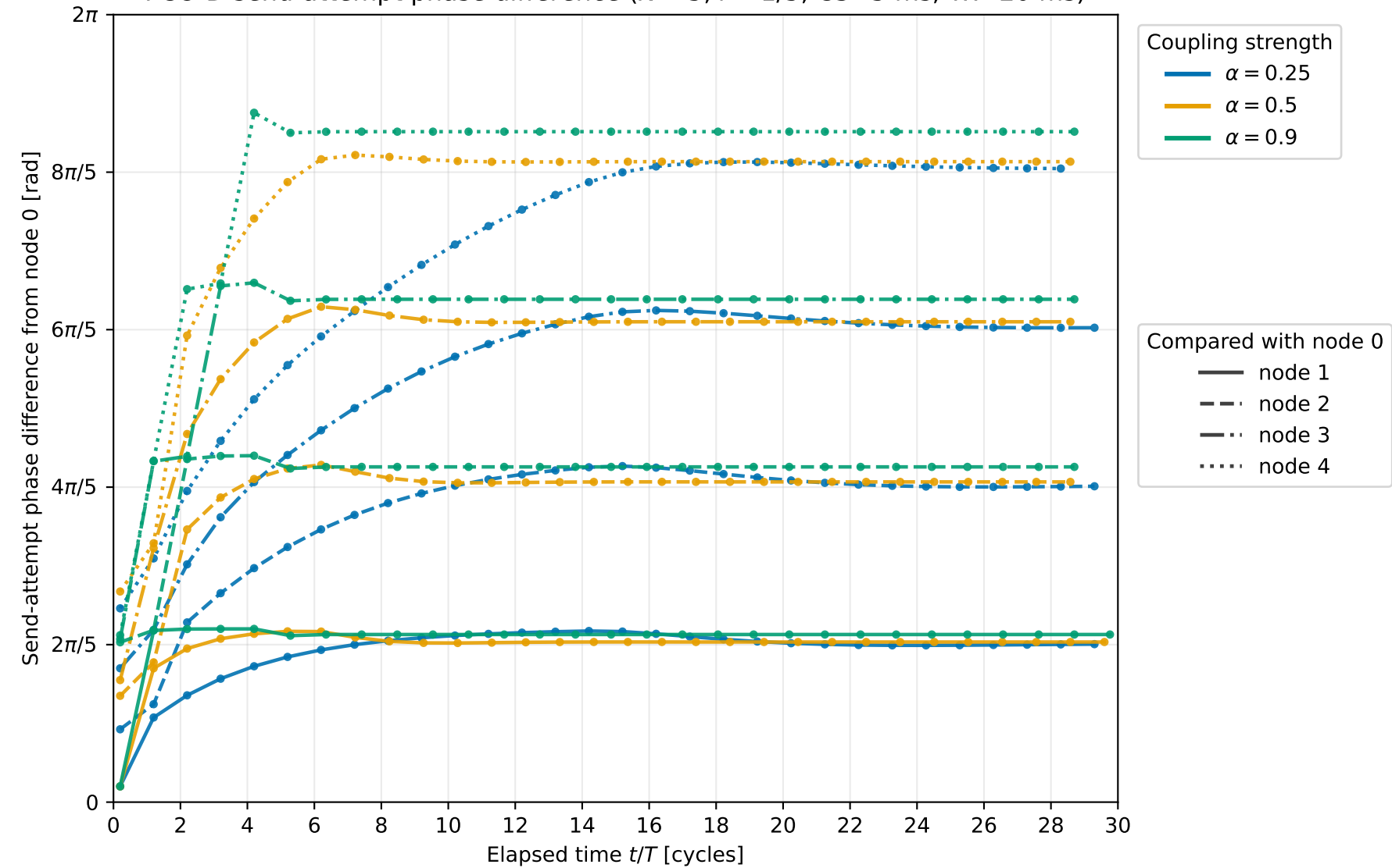
PCO-D send-attempt phase difference ( N = 5 , r = 1/5 , CS=5 ms, Tx=20 ms)
