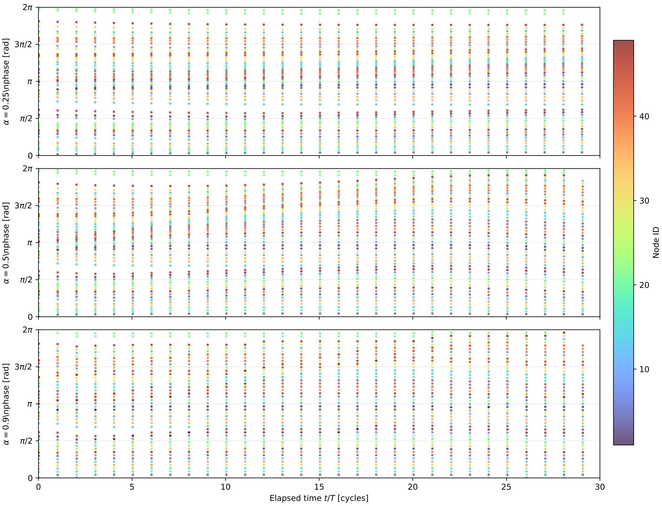
PCO-D send-attempt phase difference from node 0 ( N = 50 , r = 0.02 , T = 10000 ms, CS = 5 ms, T_x = 20 ms)
