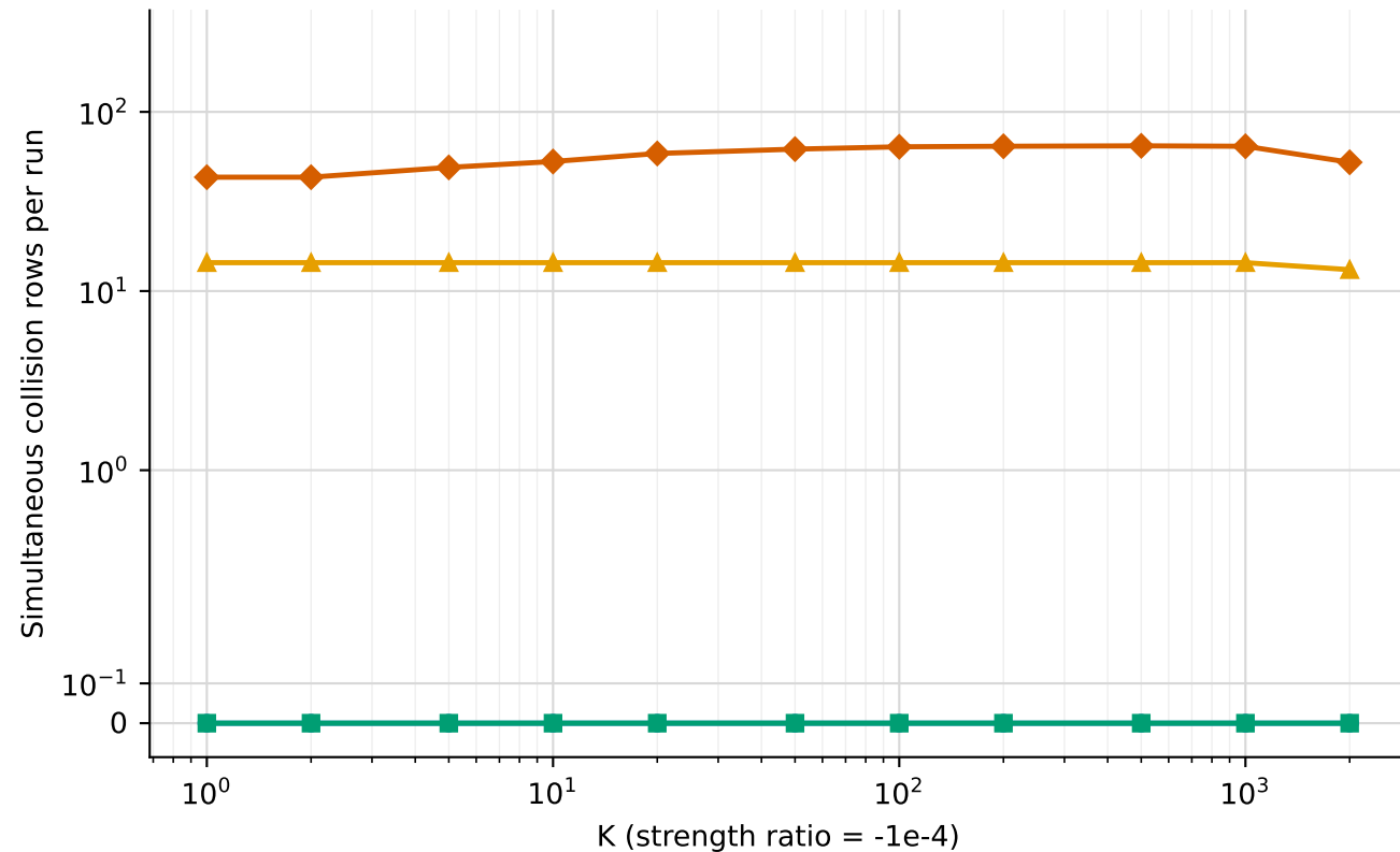
Kuramoto based
