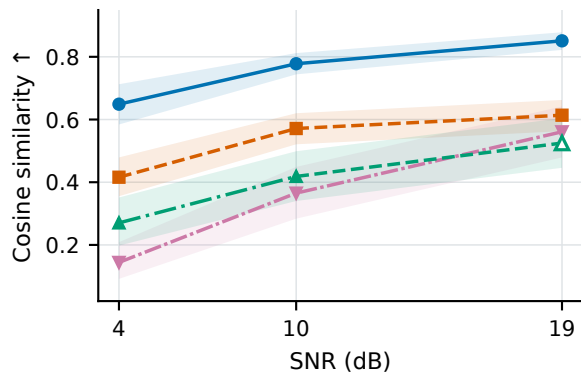
(c) DINOv2-L
