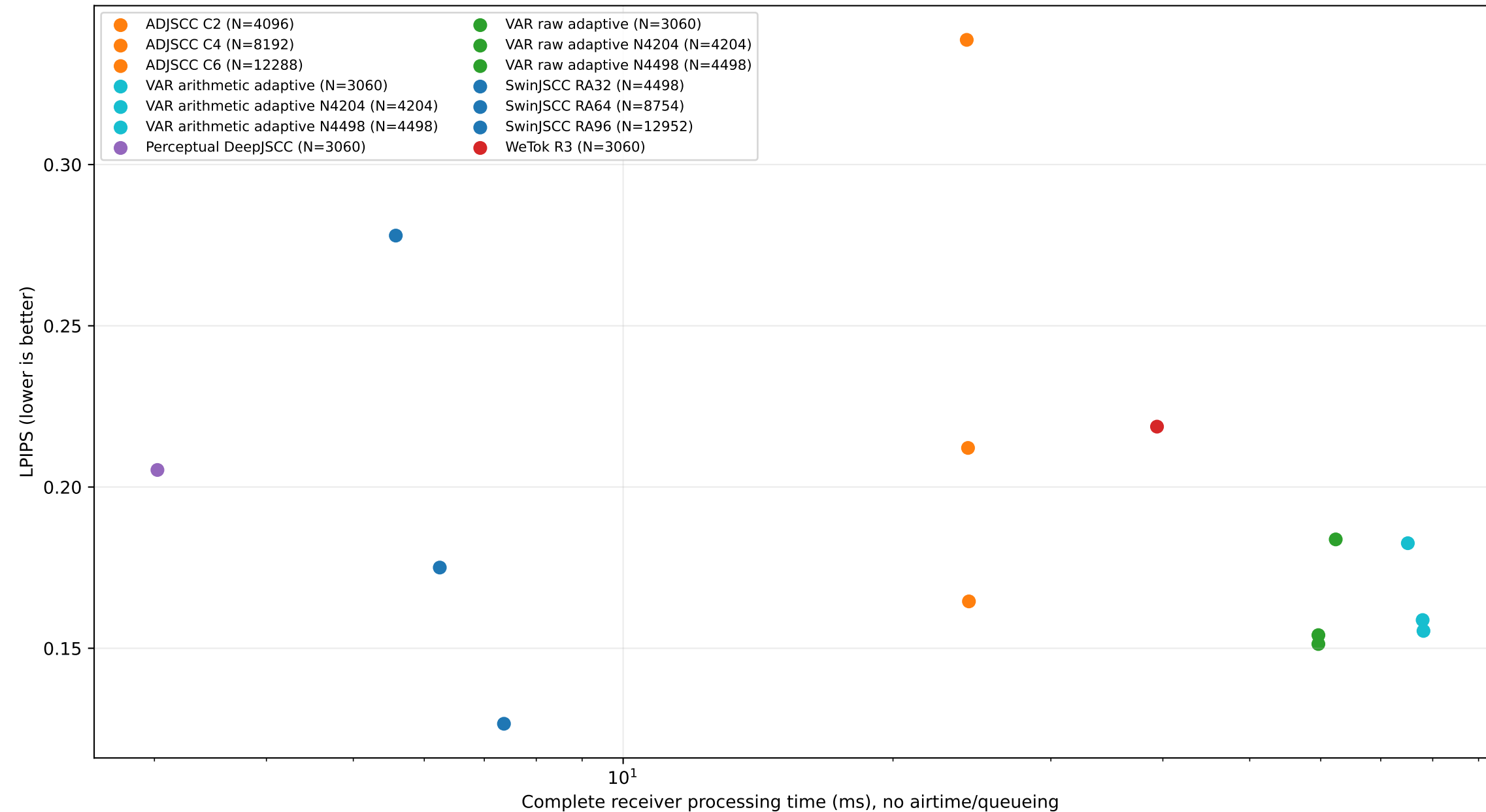
Primary1/4/7dB: measured quality vs processing cost, different budgets labelled
