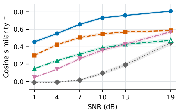
(c) DINOv2-L
