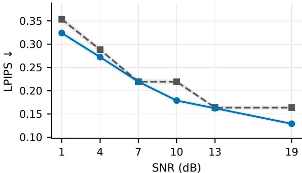
Complete-scale raw + VAR Partial-scale raw + VAR (NeST-Com) LPIPS-Alex
