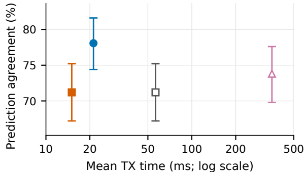
ConvNeXt prediction agreement
