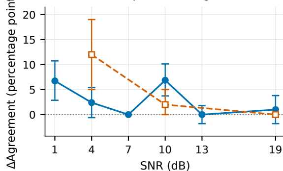
ConvNeXt prediction agreement
