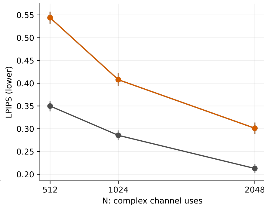
16QAM, 1 dB | 100 sources x 3 noise repeats | measured points only
