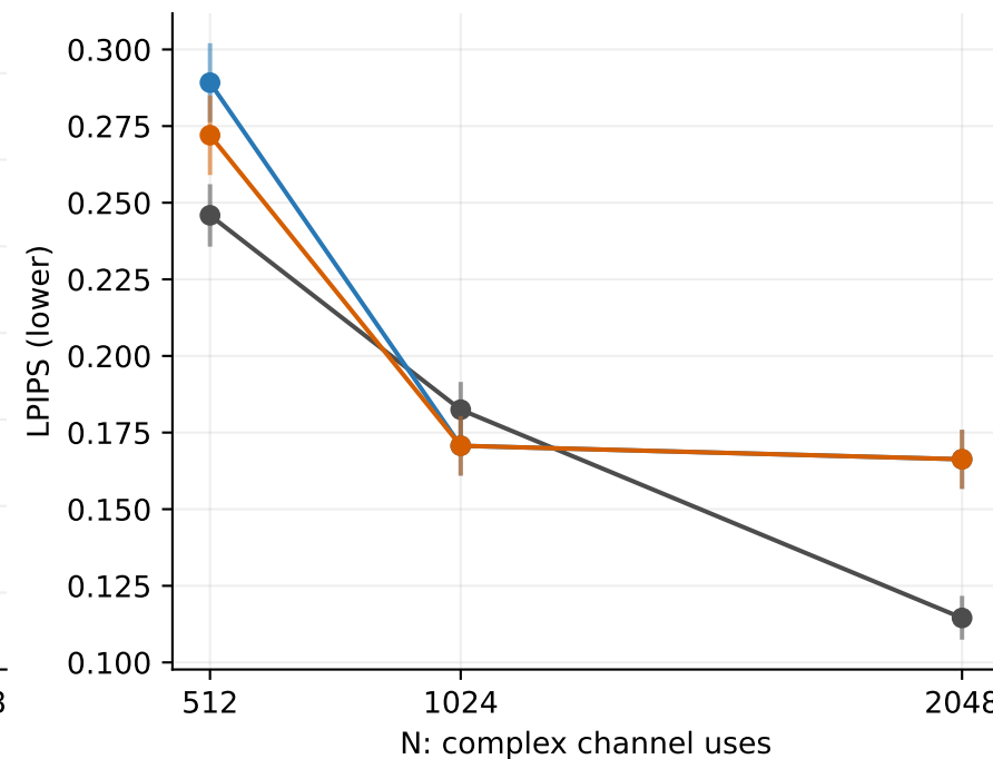
16QAM, 13 dB | 100 sources x 3 noise repeats | measured points only
