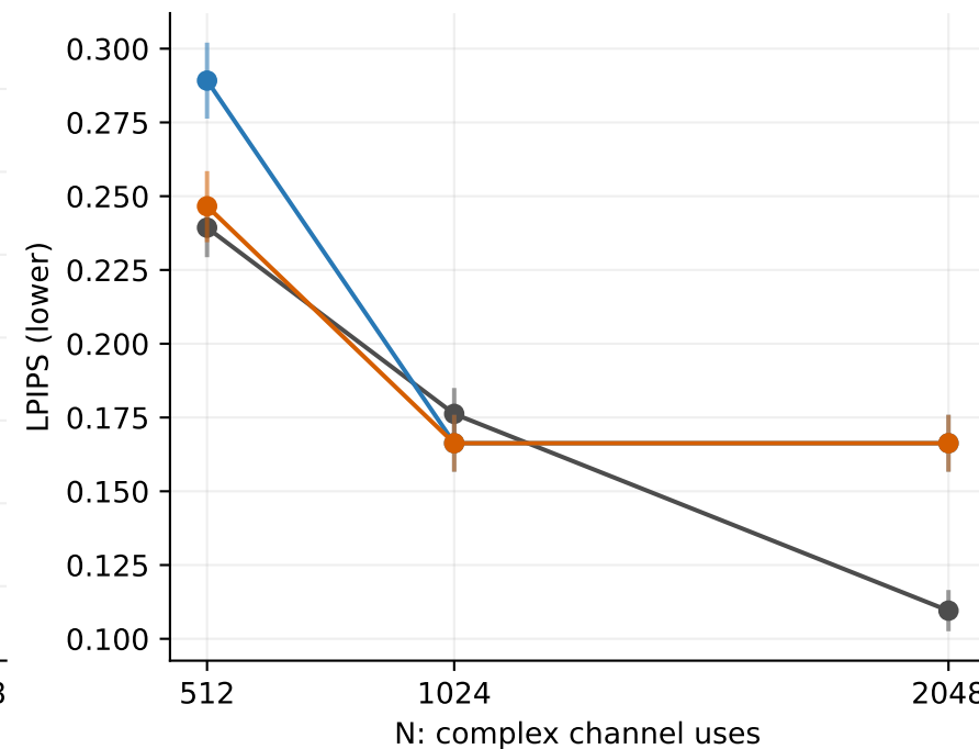
16QAM, 19 dB | 100 sources x 3 noise repeats | measured points only
