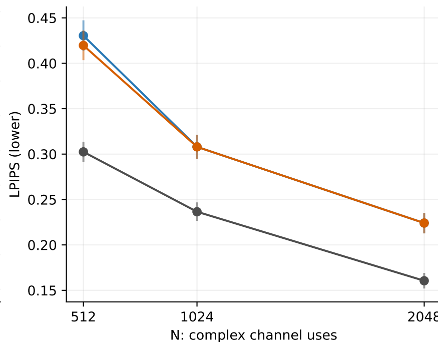
16QAM, 4 dB | 100 sources x 3 noise repeats | measured points only
