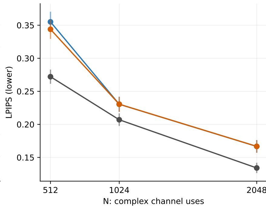
16QAM, 7 dB | 100 sources x 3 noise repeats | measured points only
