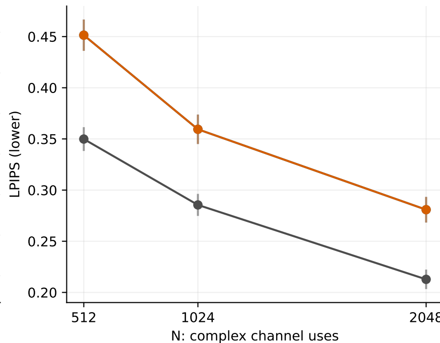
QPSK, 1 dB | 100 sources x 3 noise repeats | measured points only
