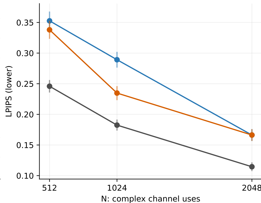
QPSK, 13 dB | 100 sources x 3 noise repeats | measured points only
