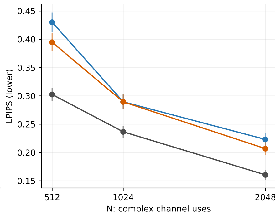
QPSK, 4 dB | 100 sources x 3 noise repeats | measured points only
