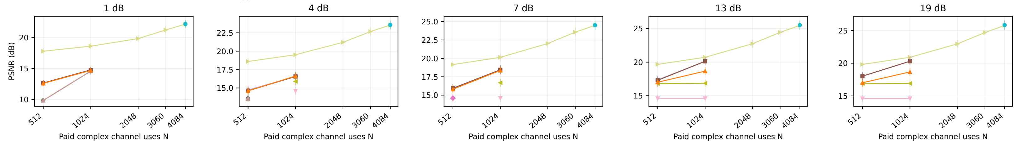
Same Dc, paid class label; QPSK, E = 2N; P is unconditional
