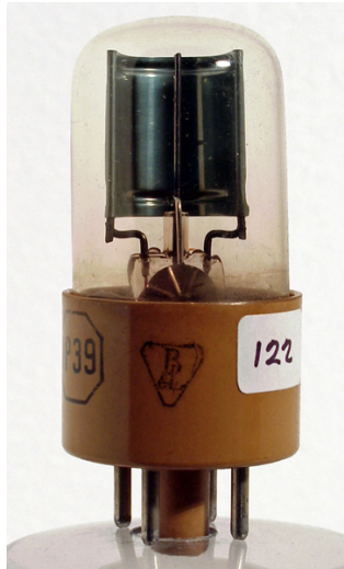
Figure 4: The 1P39 photoelectric tube inside of the Planck's constant apparatus. (The Value Meuseum, 2013) [6]
