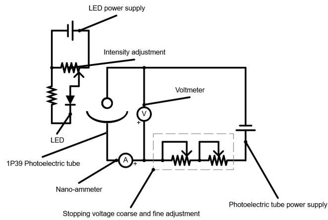
Figure 1: Diagram for the internal circuitry of the apparatus
