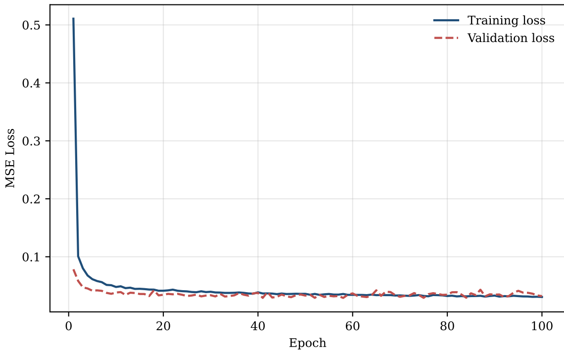
AI-ChannelNet Training and Validation Loss
