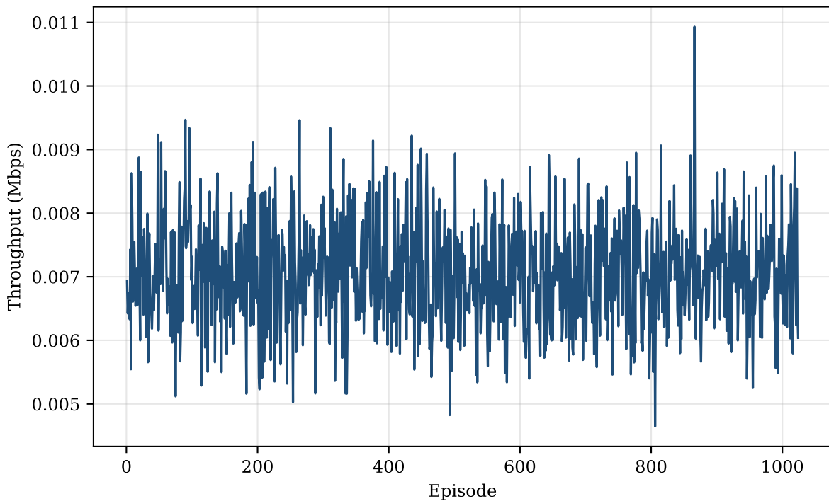
PPO Scheduler Throughput
