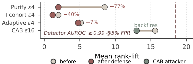
(b) Layered defense ( n = 500 )
