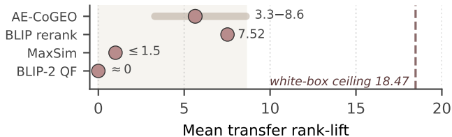
(a) Transfer below ceiling ( n = 498 )
