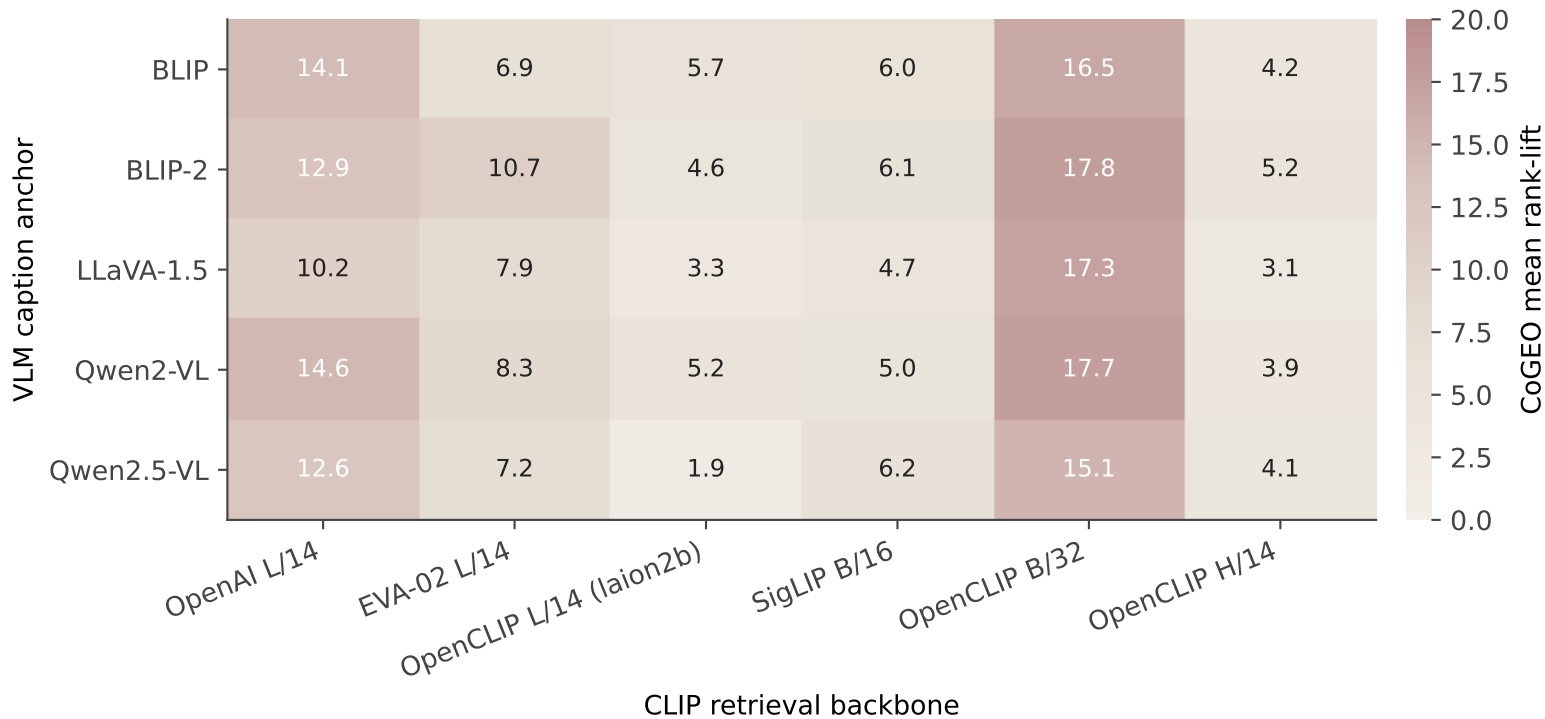
CoGEO rank-lift across 5 VLM anchors × 6 CLIP backbones (ESCI 491 ASINs, \varepsilon = 16/255 )
