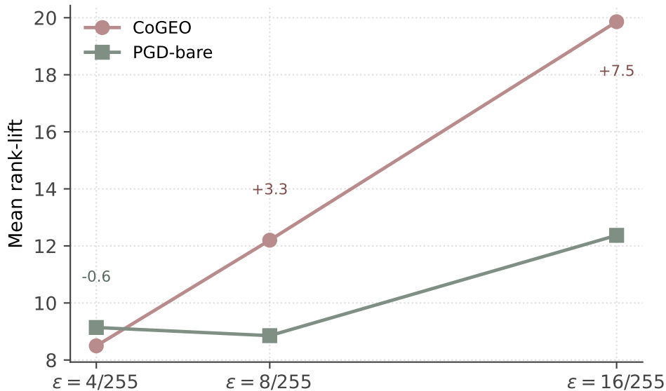
Perturbation budget sweep (ESCI 491, ViT-L/14)
