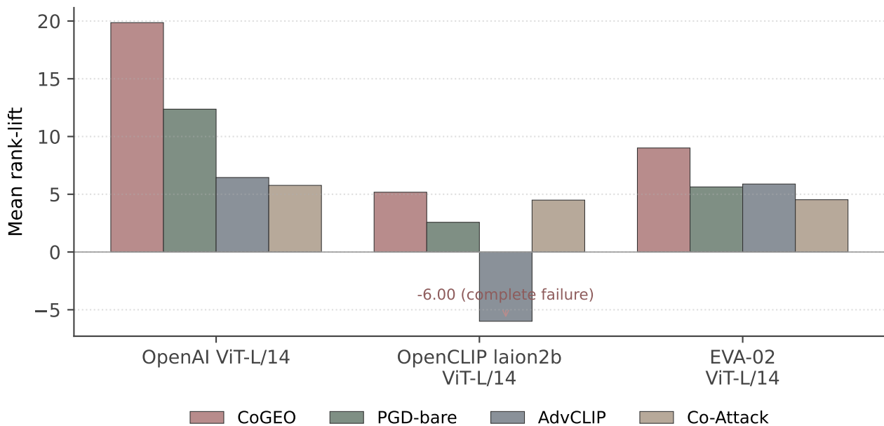
Cross-backbone four-way comparison (ESCI 491, \varepsilon = 16/255 , 224 \times 224 )
