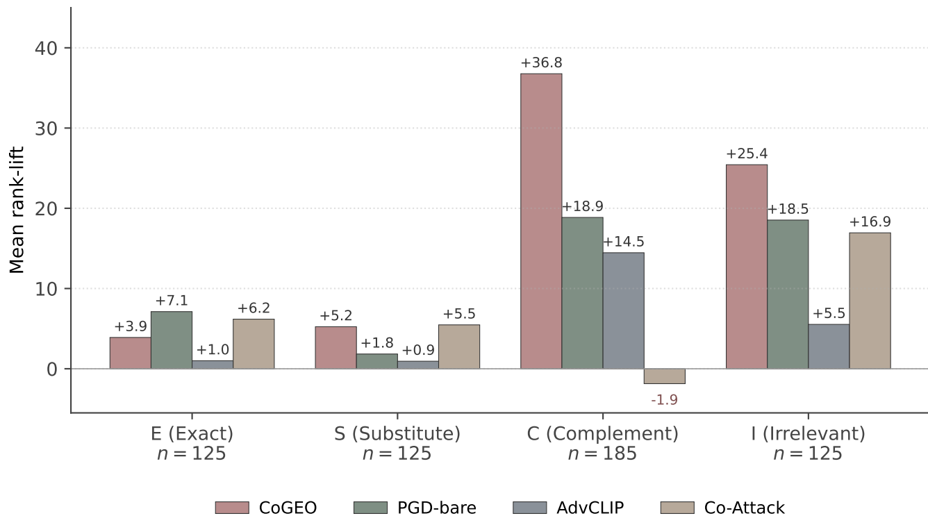
Per-cohort rank-lift on the 560-pair ESCI manifest (OpenAI ViT-L/14, \varepsilon = 16/255 )
