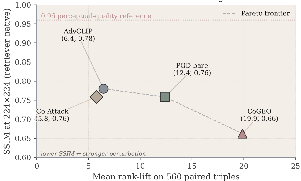
Stealth-lift Pareto across four CLIP-targeted attacks
