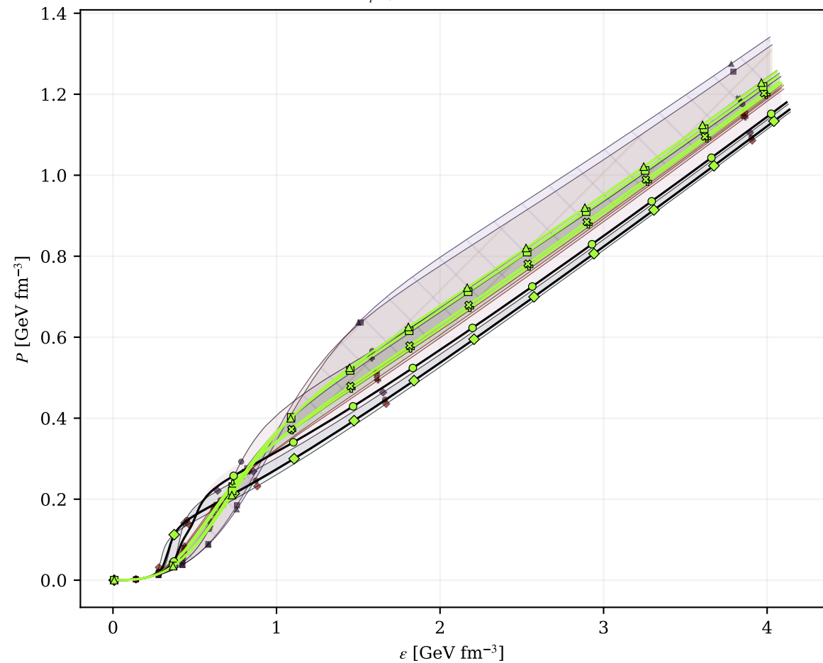
All six models, \Lambda = 300 MeV: 200 \leq K_0 \leq 350 MeV Central line: K_0=275 MeV (interpolated display guide); markers: models; black lines: vdW repulsion. b_{pn} \neq b_n , L = 58.9 MeV
