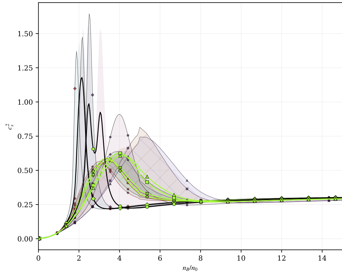
All six models, \Lambda = 300 MeV: 200 \leq K_0 \leq 350 MeV Central line: K_0=275 MeV (interpolated display guide); markers: models; black lines: vdW repulsion. b_{pn} \neq b_n , L=58.9 MeV
