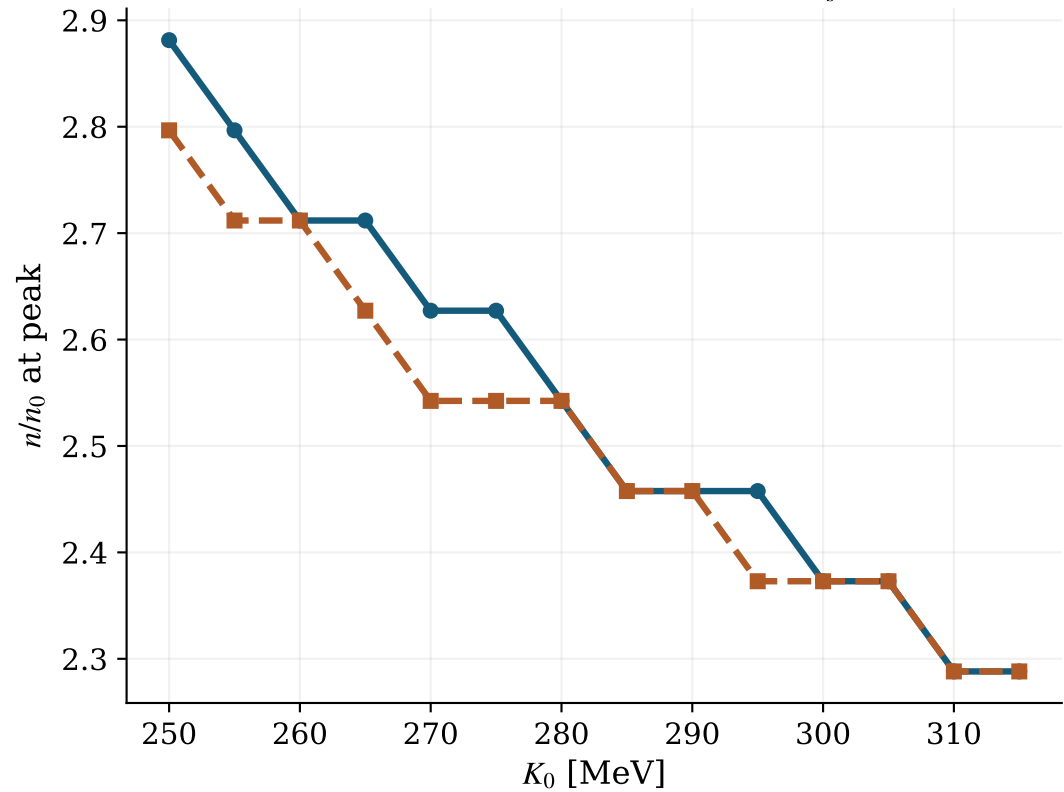
Density at the beta-equilibrium v_s^2 peak
