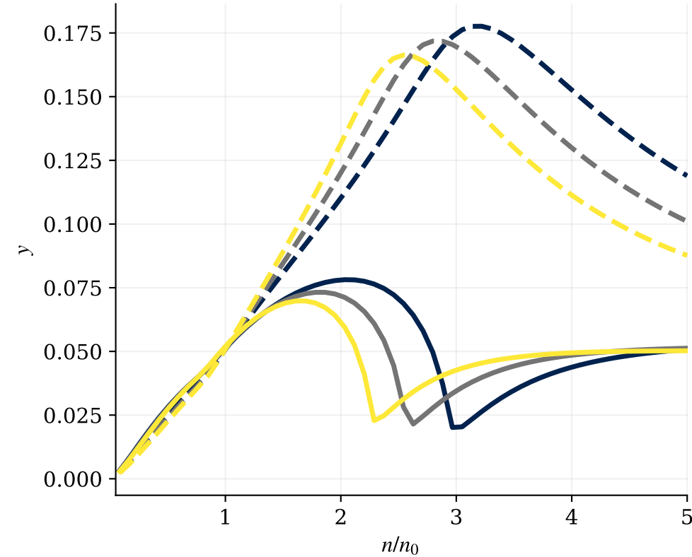
Beta-equilibrium \varepsilon/\rho_B - m_N
