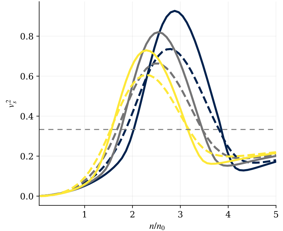
Postprocessed beta v_s^2 (window=29, degree=3)
