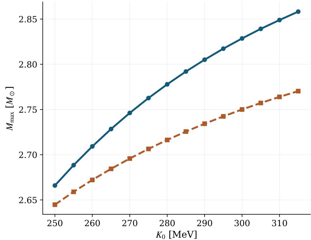
Neutron-star maximum mass
