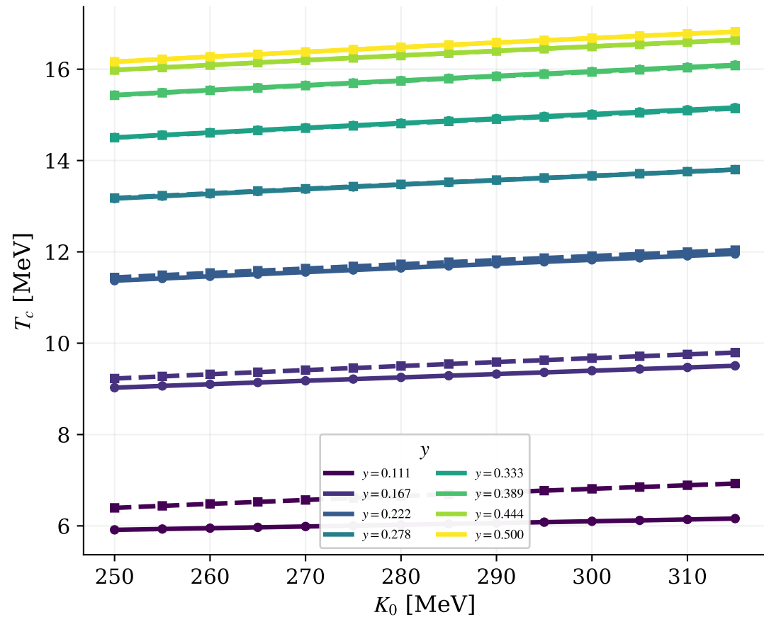
T_c versus K_0
