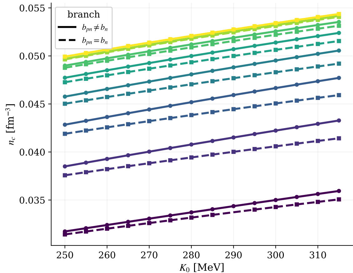
n_c versus K_0
