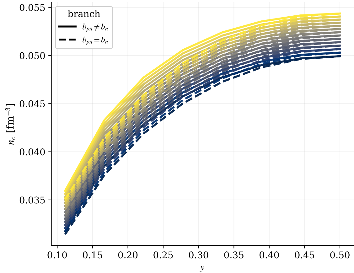
n_c versus fixed proton fraction
