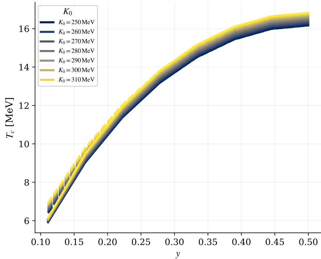
T_c versus fixed proton fraction
