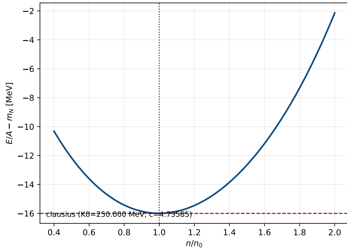
Hadronic Binding Curve
