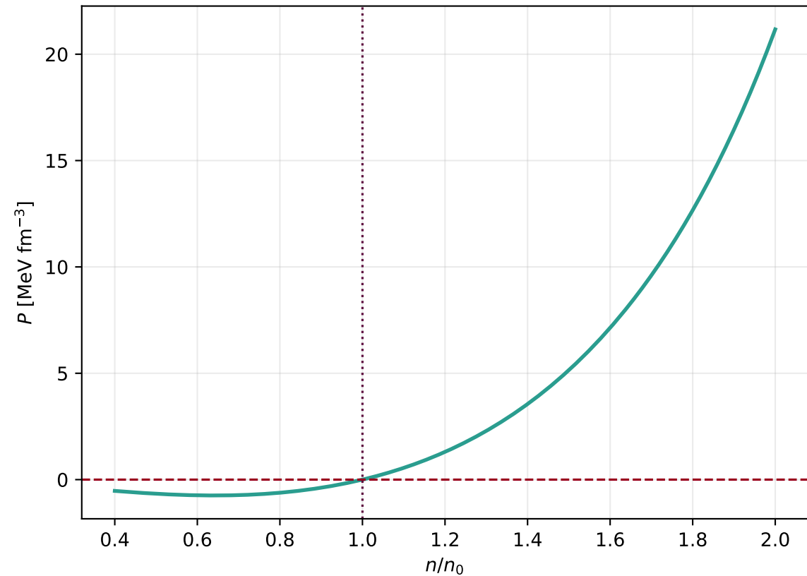
Hadronic Pressure
