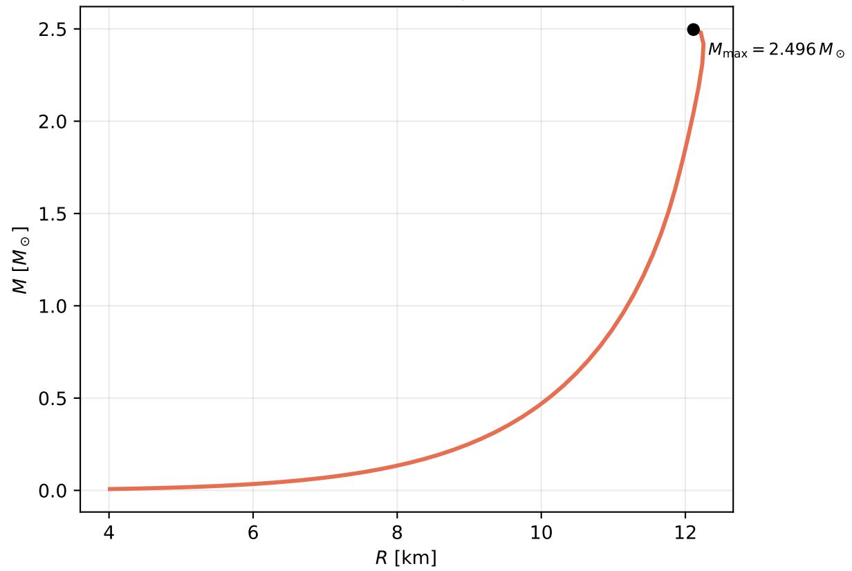
Mass-Radius Sequence
