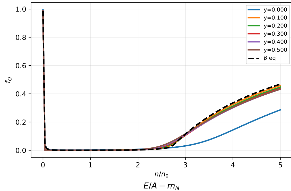
Quark Fraction
