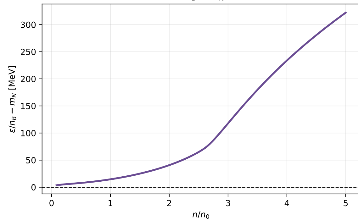
\varepsilon/n_B - m_N
