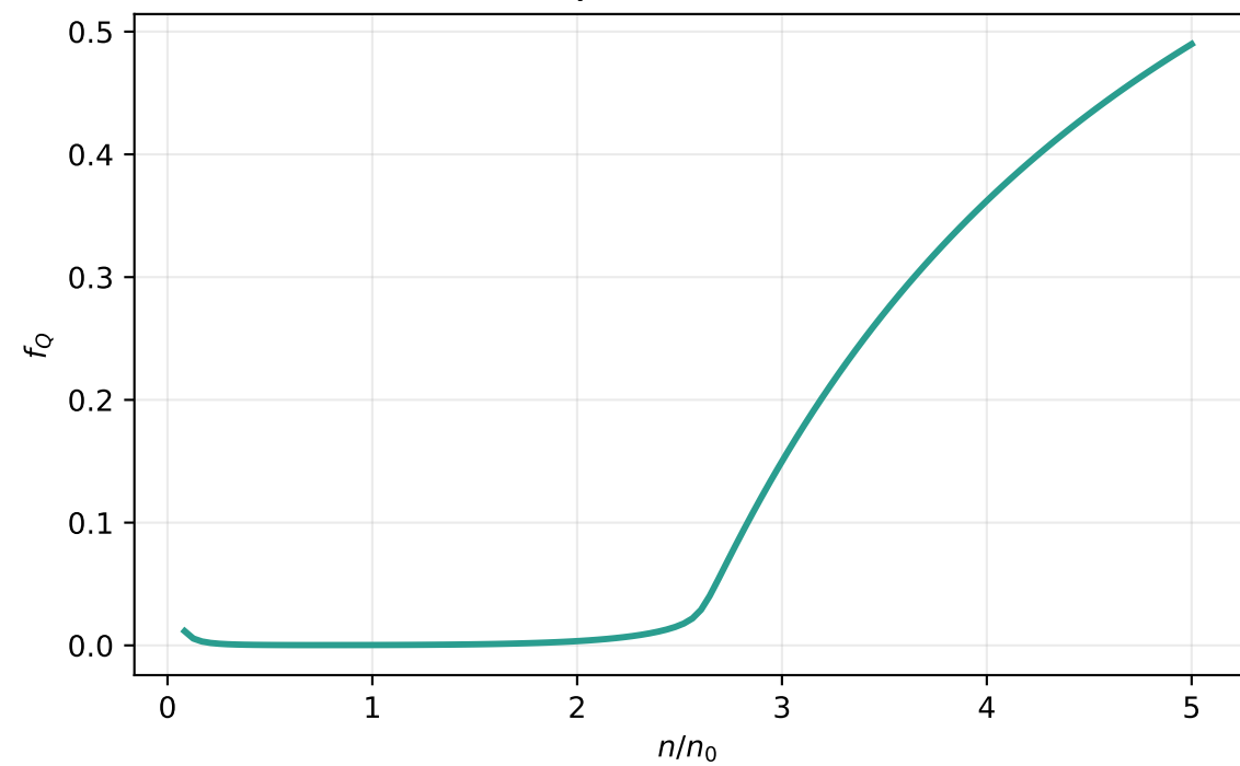
Quark Fraction
