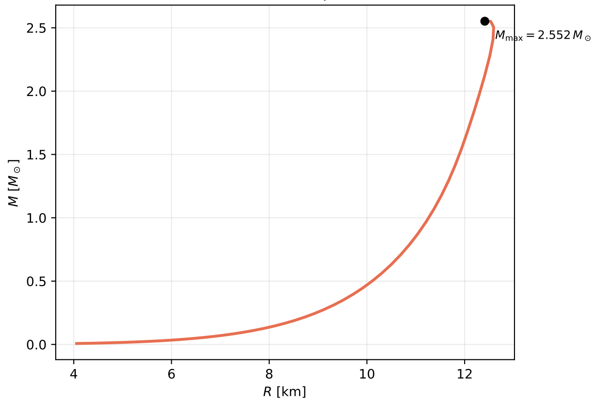
Mass-Radius Sequence
