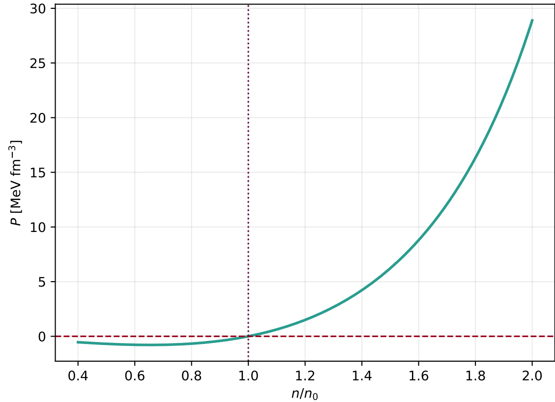
Hadronic Pressure
