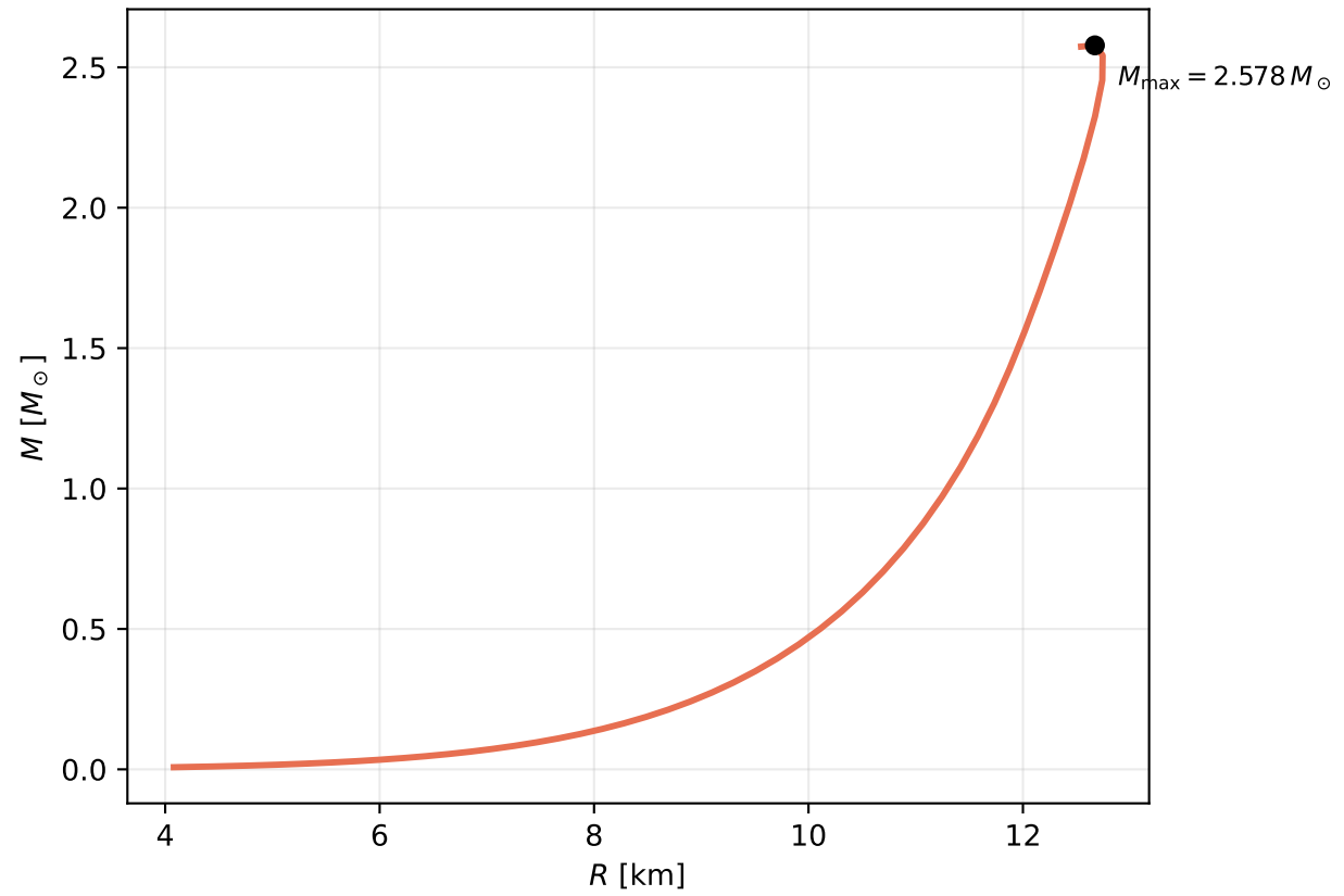
Mass-Radius Sequence
