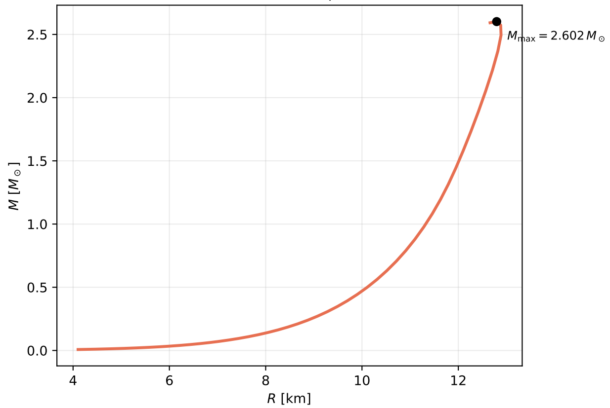
Mass-Radius Sequence
