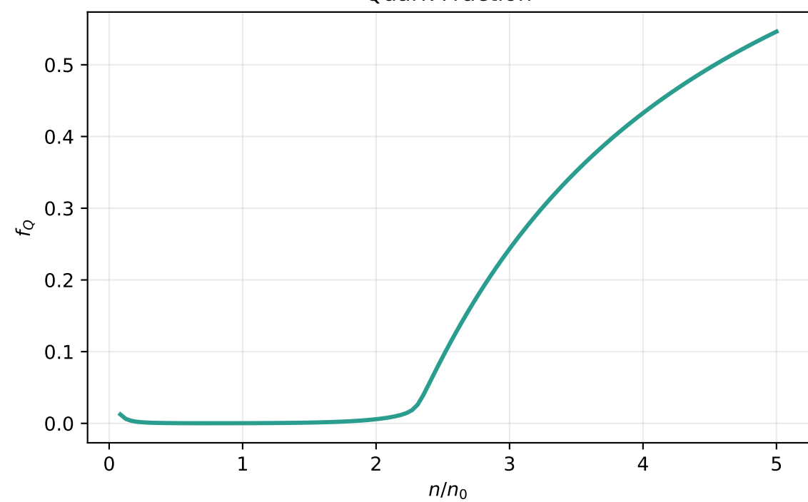
Quark Fraction
