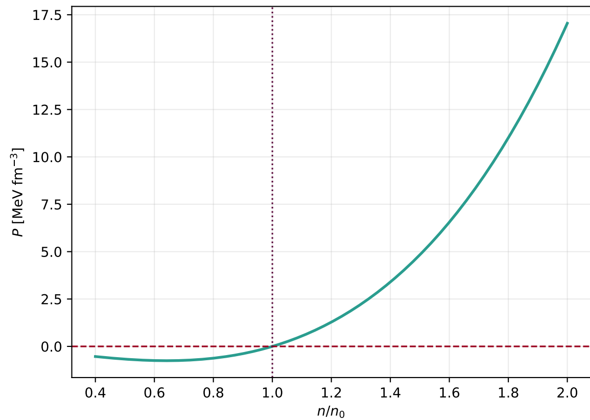
Hadronic Pressure
