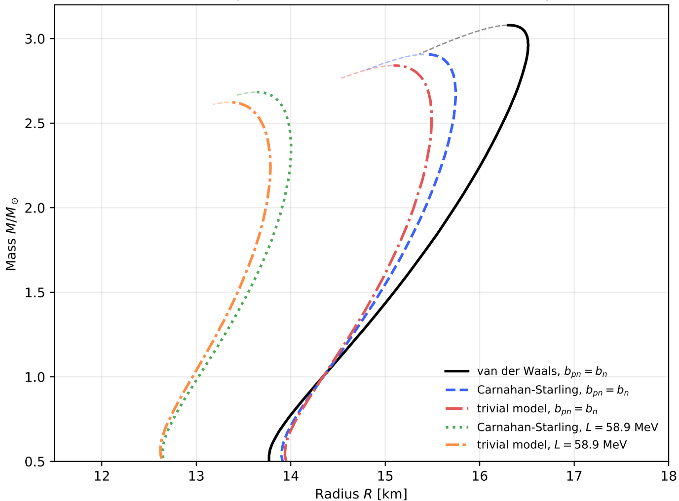
Guided beta-equilibrium models: TOV mass-radius sequences
