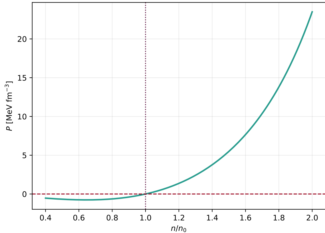
Hadronic Pressure
