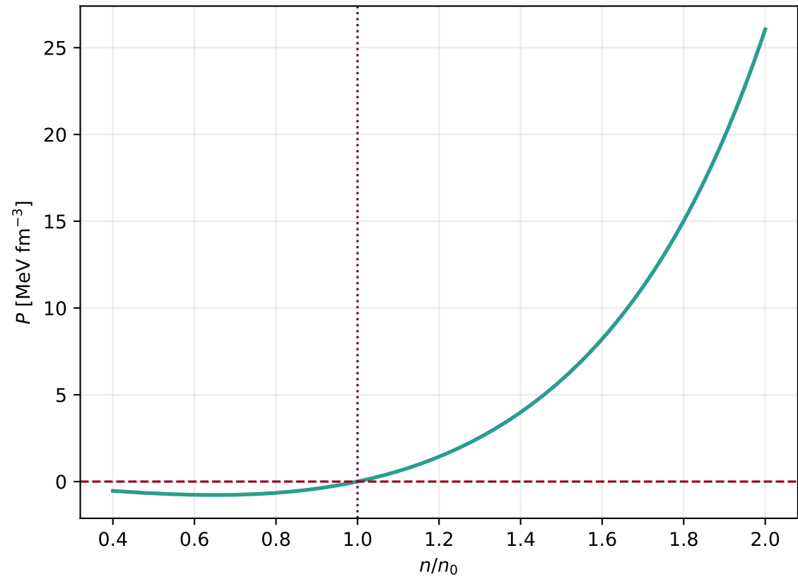
Hadronic Pressure
