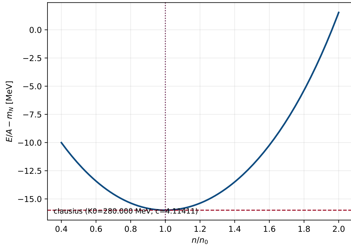
Hadronic Binding Curve
